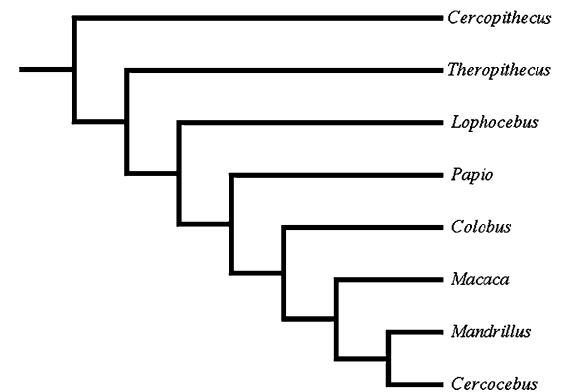
Fig. 7. Most parsimonious cladograms derived from mixed-sex dental characters that remain significantly correlated with the geometric mean after size-correction.
