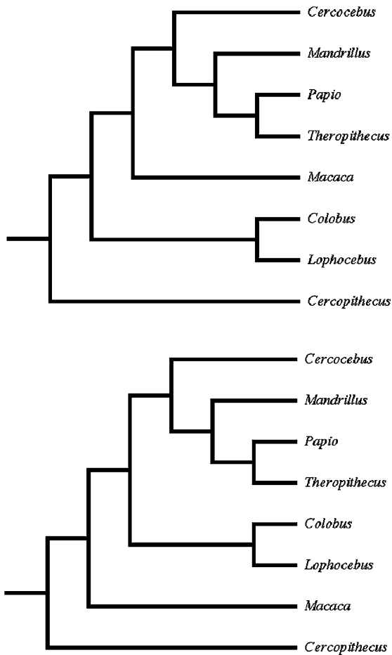
Fig. 2. Most parsimonious cladograms derived from mixed-sex high-strain characters.
