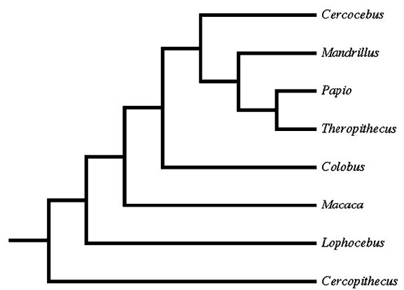
Fig. 3. Most parsimonious cladogram derived from mixed-sex low-to-moderate-strain characters.
